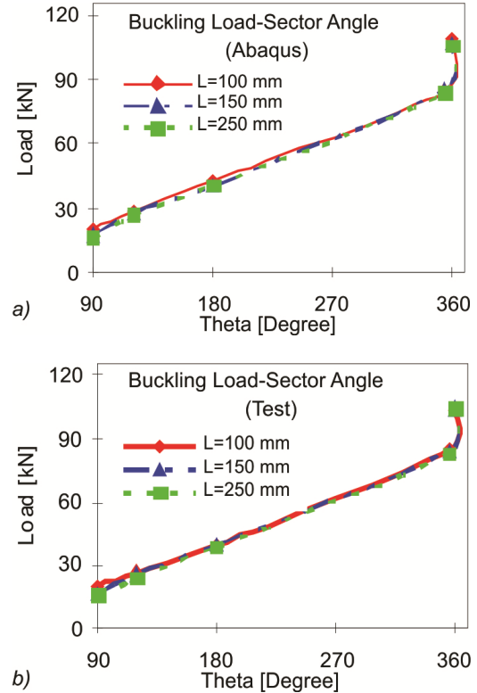
Fig. 12. Buckling load in terms of the sector angle for different lengths (simply supported): a) numerical analysis, b) experimental test
