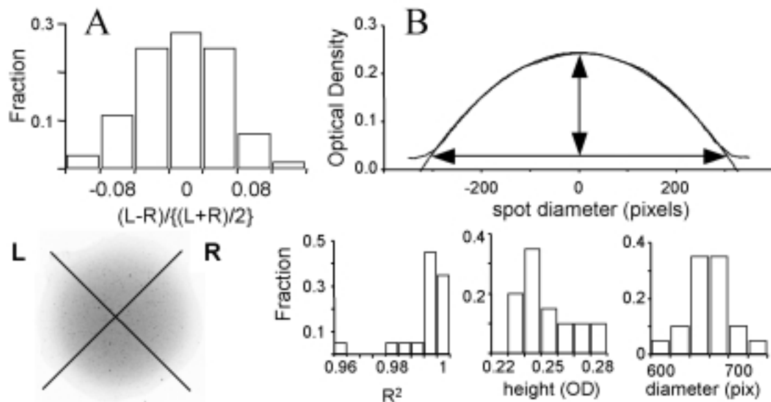
Fig. 1. Shape of the gelatin calibration spots. A. Gelatin spot with two orthogonal profiles and frequency distribution of the difference in profile length. B. Fit of a parabola to the cross-sectional profile of a gelatin spot with frequency distributions of the correlation coefficient ( R^2 ), height and diameter.
