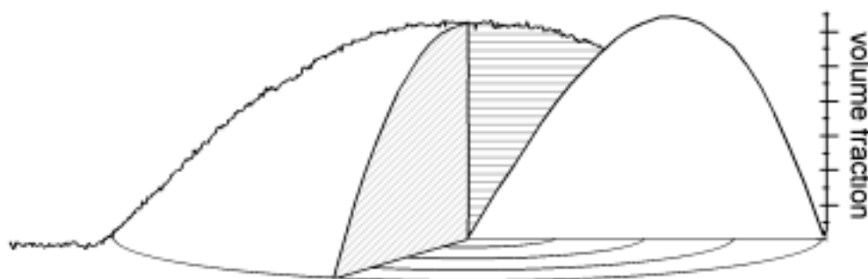
Fig. 2. A gelatin calibration spot has a circular base with a parabolic cross-section. The graph shows the distribution of the volume of the spot over concentric rings.
