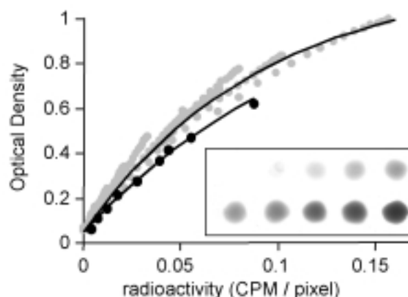
Fig. 3. Results of the measurement of mean OD of the 10 whole spots (black dots) and measurement of 15 concentric rings on each spot (gray dots). Solid lines are fitted with Eq. 2. Inset: calibration slide.
