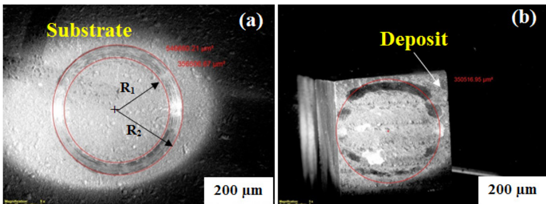
Fig. 2. Wear track of the substrate and the Ti-6Al-4V+B 4 C deposit at 2.0 kW
