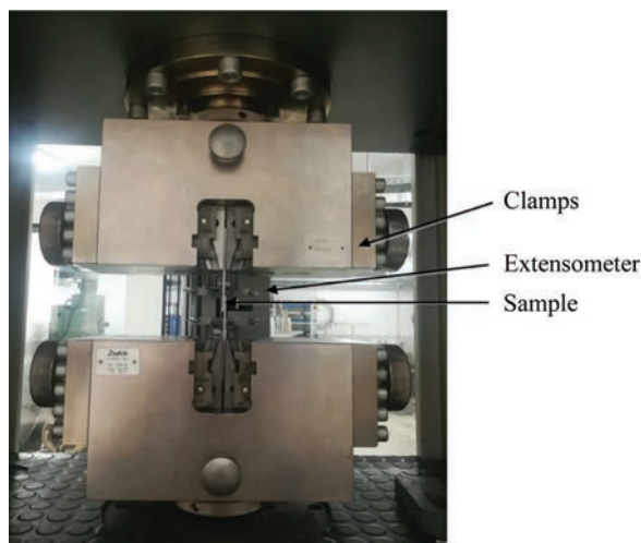
Fig. 3. Layout of the test rig
