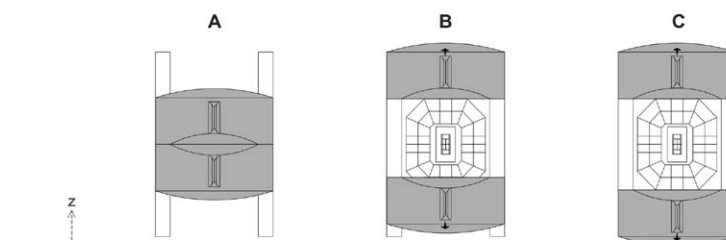
Figure 14: Ariake Colosseum sports hall; demonstration of the roof structure sliding in the longitudinal direction (A - closed, B - half-open, C - open).
