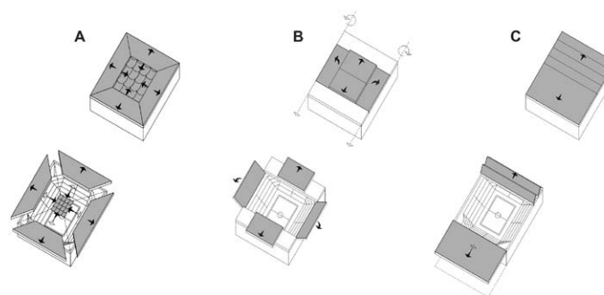
Figure 24: A. Retraction of entire roof structure with rigid elements and membrane (sliding system, folding system) B. Retraction of individual rigid roof parts (sliding system, rotating system); C. Retraction of entire rigid roof structure (sliding system, folding system).
