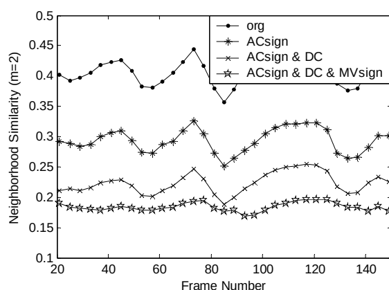
Figure 5: Neighborhood similarity of multi-level encryption.
