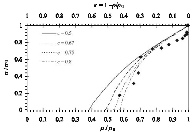
Figure 6: Calculated relationships between the relative conductivity \sigma/\sigma_0 and the relative density \rho/\rho_0 or porosity \varepsilon for different parameters c ; (solid, dashed and dotted lines as described by Mizusaki et al. 25 ) and the observed trend of the measured data (◆ LSM tablets). The relative shape parameter c determines the contribution of the two sine-waves in describing the shape of the cross-section of the particle during sintering.
