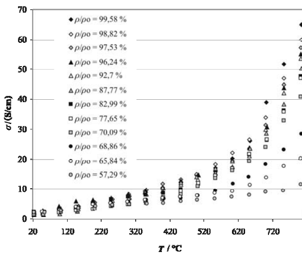
Figure 5: Specific conductivity vs. temperature for a series of LSM elements cermet with various relative densities
