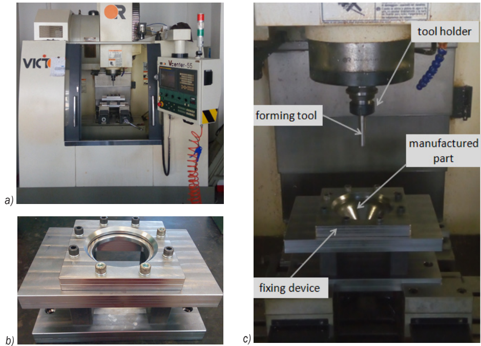
Fig. 9. Setup used for ISF process implementation; a) Victor Vcenter-55 CNC milling machine; b) sheet metal fixing device; c) elements for ISF implementation, adapted from [33]
