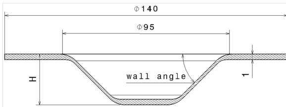
Fig. 6. Experimental frustum of a cone
