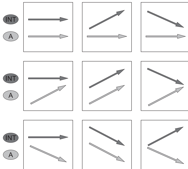
FIGURE 4.2 Measurement Method as Pattern Recognition II: Development of Scientific Fields
