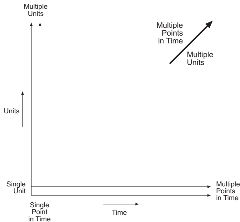
FIGURE 5.15 The N x T Scope for Morphological Comparisons
