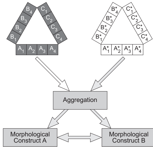
FIGURE 5.7 The Morphological Aggregation Procedure
