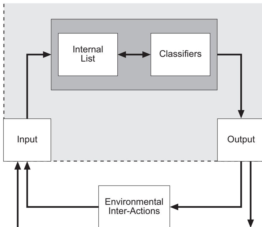
FIGURE 2.1 A Scheme for a GA-Classifer System
