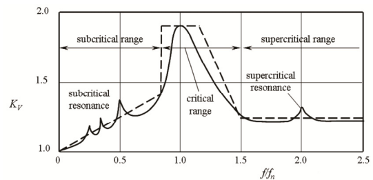
Fig. 2. Dynamic factor K_v [3] and approximation of gear dynamic forces and vibration
