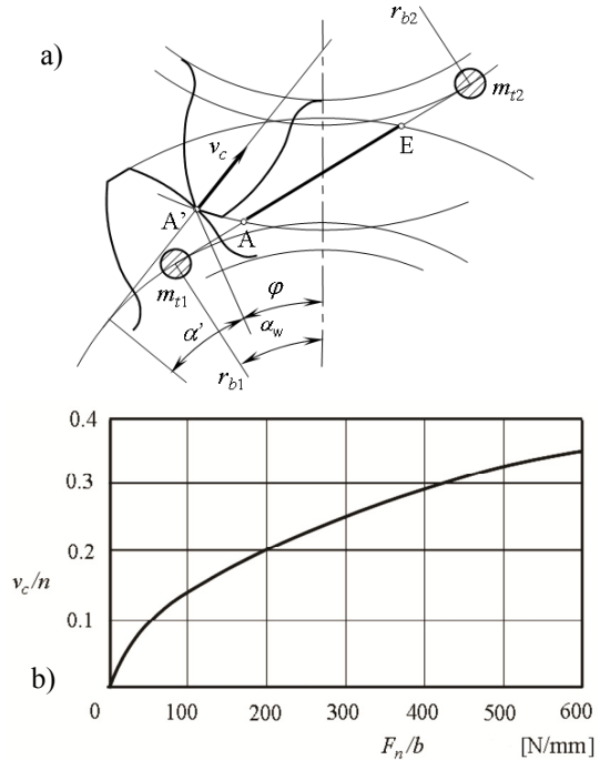
Fig. 3. Teeth collision: a) addendum collision, b) relative speed of addendum collision for chosen gear parameters
