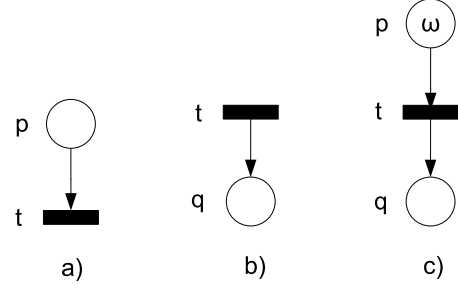
Figure 3: Transitions without input/output
