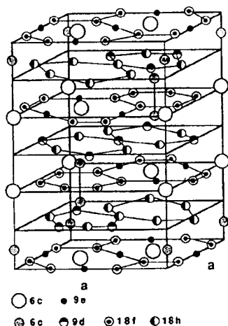
Figure 1: Rhombohedral crystall structure of \text{Nd}_2\text{Fe}_{17-x}\text{Al}_x Slika 1: Romboedrična kristalna struktura \text{Nd}_2\text{Fe}_{17-x}\text{Al}_x
