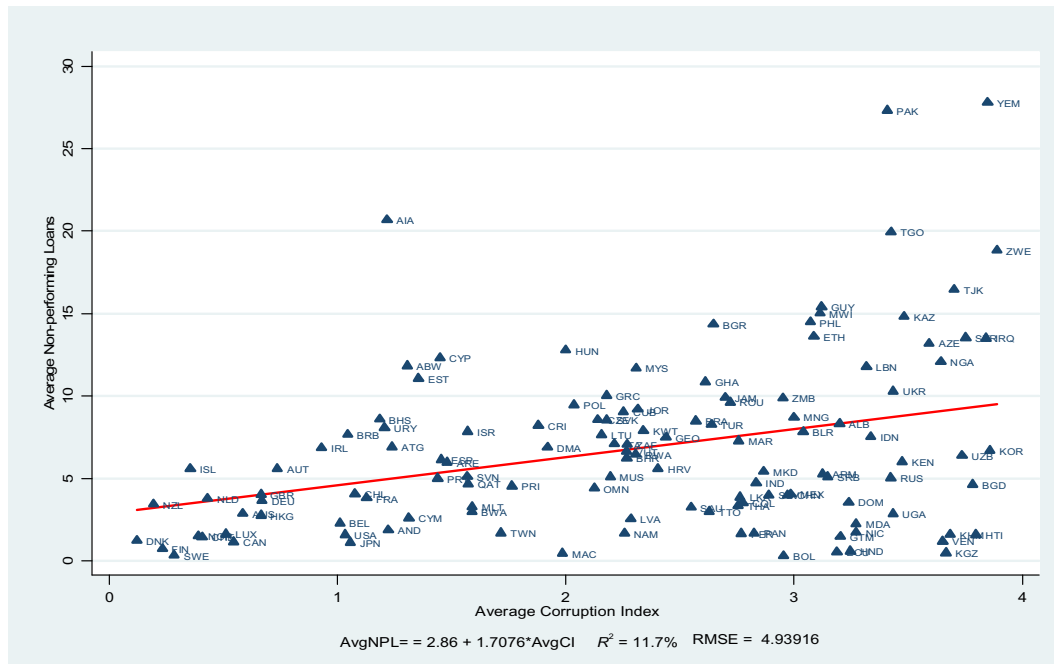
Fig. 1. Plot of the average corruption index and NPLs. Note: We use standard regression equation as an estimation method. The horizontal axis on the graph represents the average corruption index (AvgCI) and the vertical axis (AvgNPL) represents the average NPLs where the average is computed for different countries. Source: World Bank and Fitch Connect.
