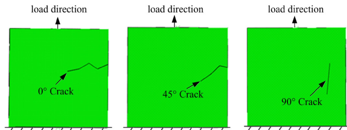
Fig. 22. Location of the crack angle in the WC particles and model load under a tensile displacement
