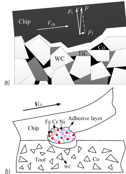
Fig. 4. The adhesion layer is removed in the form of chips; a) forces of the cutting tool in the cutting process, and b) schematic diagram of the formation of tool-chip adhesion
