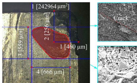
Fig. 5. Bond breakage of the tool
