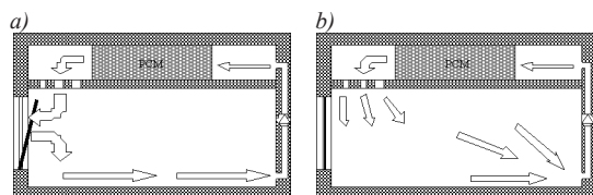
Fig. 1. Principal function of PCM "free cooling system"; a) night time, b) day time
