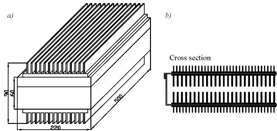
Fig. 3. a) Shape and b) cross section of the cold storage
