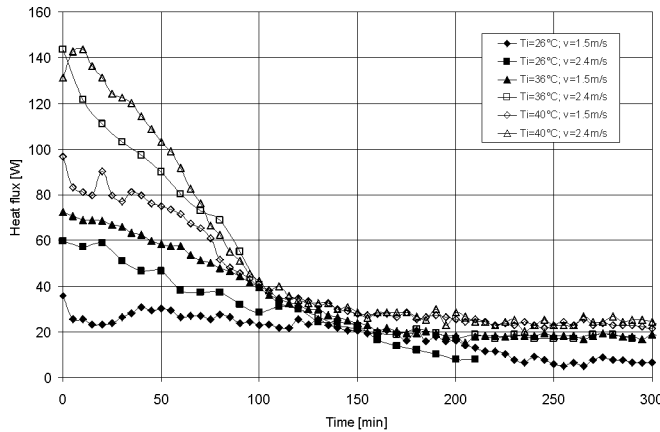
Fig. 5. Heat flux of the cold storage at different inlet air temperatures and airflows
