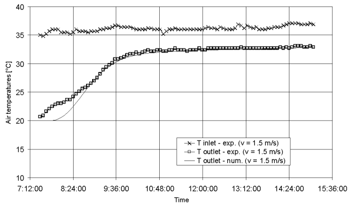
Fig. 8. Comparison of experimental and numerical values of air temperatures
