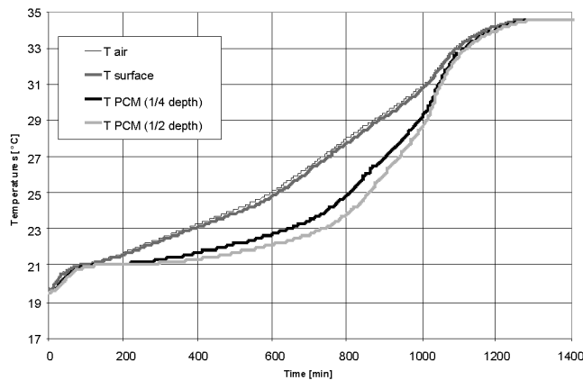
Fig. 9. Temperatures of air, surface and PCM in middle cross section
