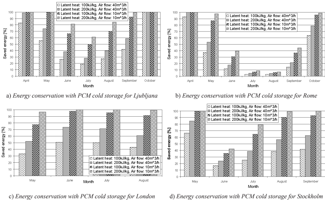
Fig. 10. The share of saved energy for different European cities
