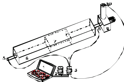
Fig. 2. Testing line scheme for measuring daily cold storage efficiency
