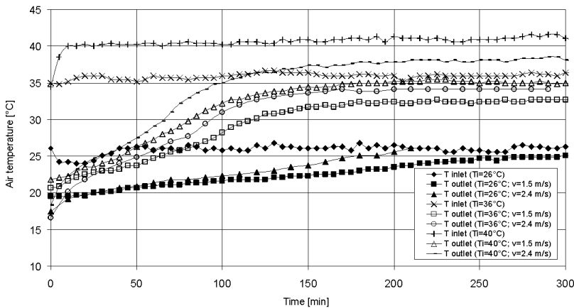
Fig. 4. Outlet air temperatures at different inlet air temperatures and airflows
