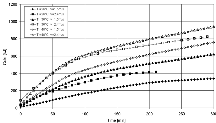
Fig. 6. Amount of cold stored in cold storage at different inlet air temperatures and airflows
