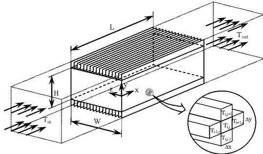
Fig. 7. Control volume of the PCM
