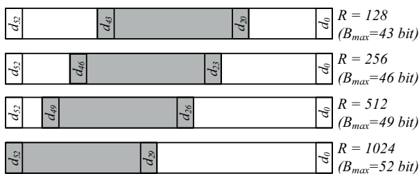
Figure 9: Truncation at last decimator according to decimation rate R
