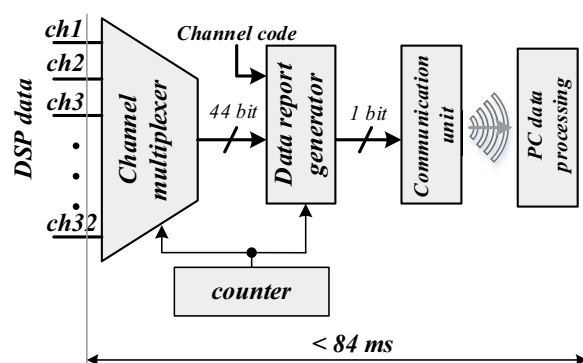
Figure 11: DSP data reporter block diagram with Communication unit
