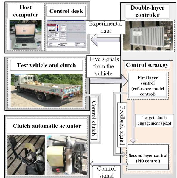
Fig. 14. Experimental setup
