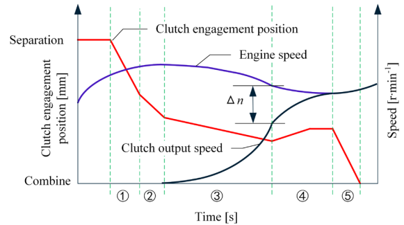
Fig. 10. Control curve of a vehicle start-up process
