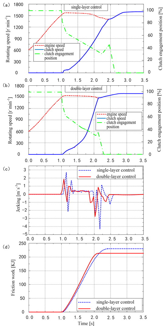
Fig. 13. Simulation results at low temperature ( -10\text{ }^{\circ}\text{C} ), a) single-layer control, b) double-layer control, c) jerking contrast, and d) friction work contrast
