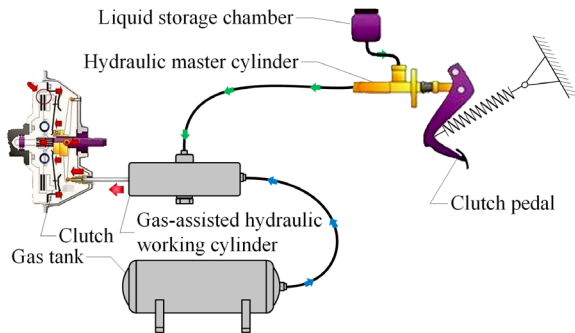
Fig. 5. Gas-assisted hydraulic clutch actuator
