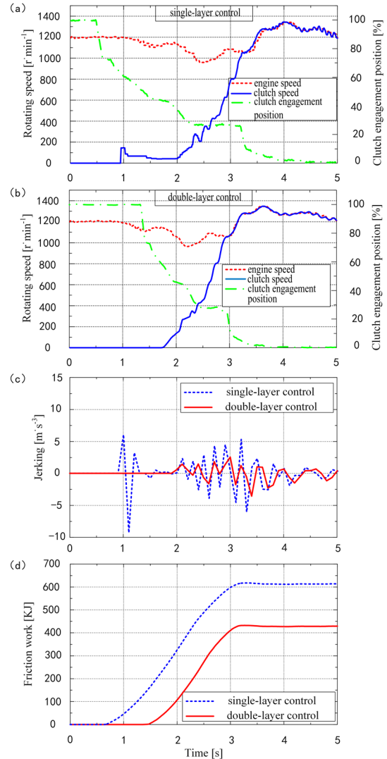
Fig. 16. Experimental results at low temperature (-10 °C), a) single-layer control, b) double-layer control, c) jerking contrast, and d) friction work contrast
