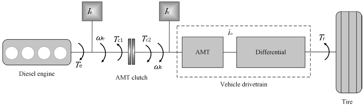
Fig. 3. Simplified model of the test vehicle's driveline
