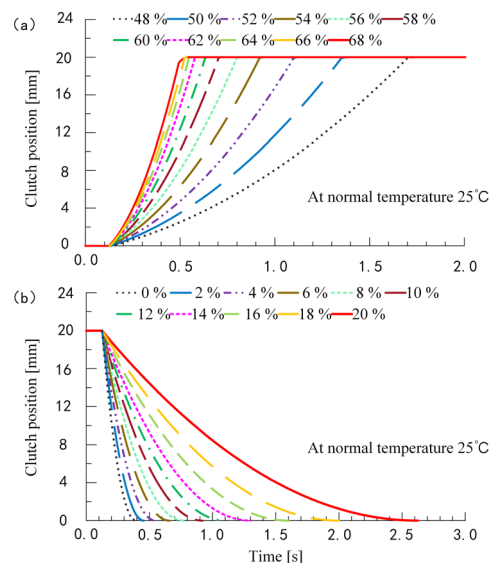
Fig. 9. Curves of a) clutch separation, and b) clutch engagement
