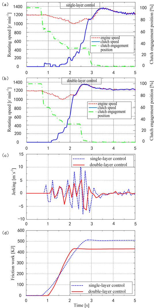
Fig. 15. Experimental results at normal temperature (25 °C), a) single-layer control, b) double-layer control, c) jerking contrast, and d) friction work contrast
