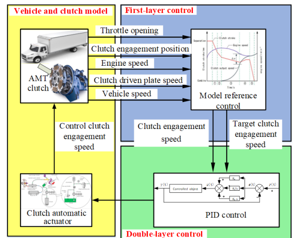
Fig. 11. Double-layer clutch control strategy
