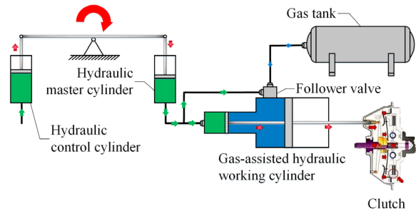
Fig. 7. Action of the automatic clutch actuator
