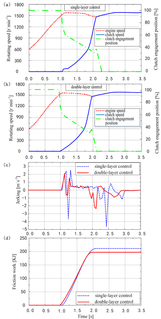
Fig. 12. Simulation results at normal temperature (25 °C), a) single-layer control, b) double-layer control, c) jerking contrast, and d) friction work contrast
