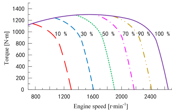
Fig. 1. Fixed throttle characteristics of a diesel engine with variable-speed governor
