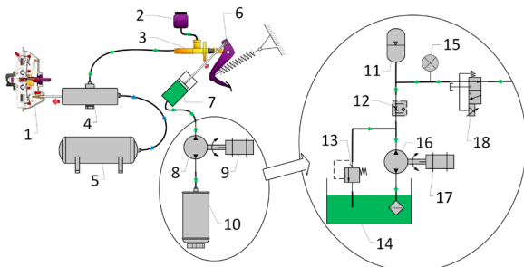
Fig. 6. Gas-assisted hydraulic automatic clutch actuator:
