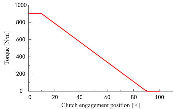
Fig. 4. Relationship between clutch output torque and clutch engagement position
