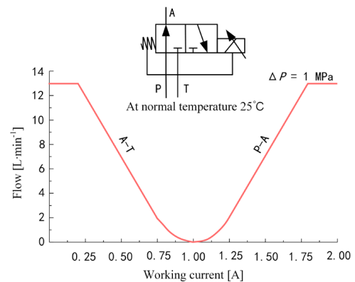
Fig. 8. Basic working characteristics of the proportional flow valve
