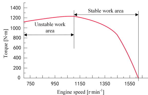
Fig. 2. Diesel engine speed-torque curve with 30 % throttle opening
