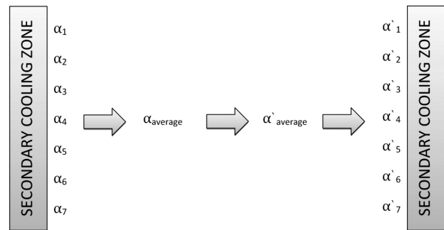
Figure 7: Diagram for a calculation of new heat-transfer coefficients 25 Slika 7: Prikaz izračuna novih koeficientov prenosa toplote 25
