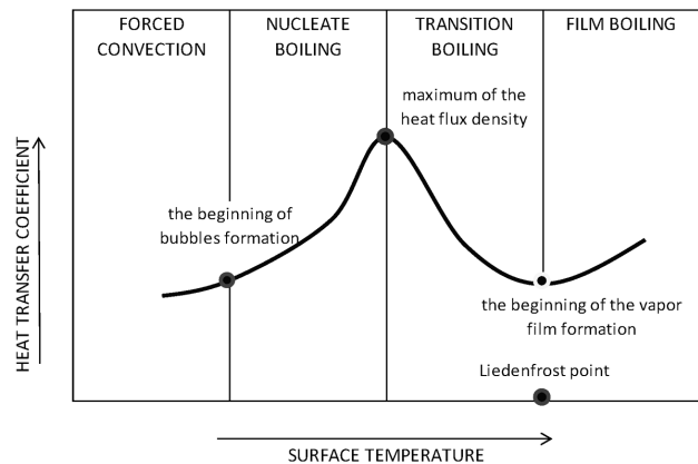
Figure 2: Flow diagram for the heat-transfer coefficient changing during the boiling process 3
