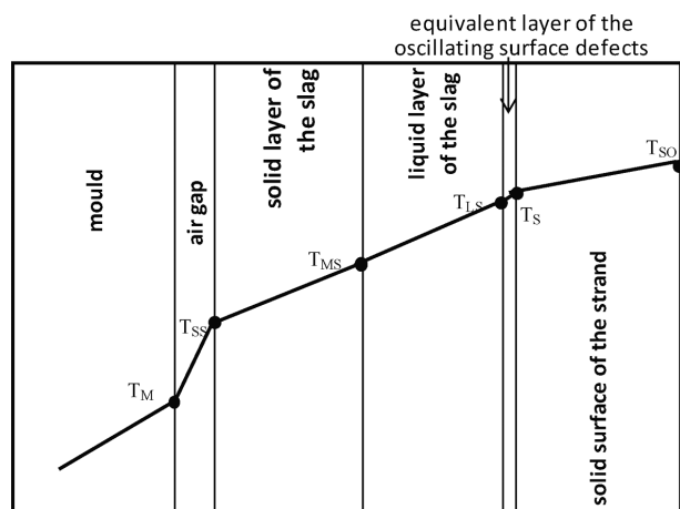
Figure 1: Structure of the layer between the mould and the shell
