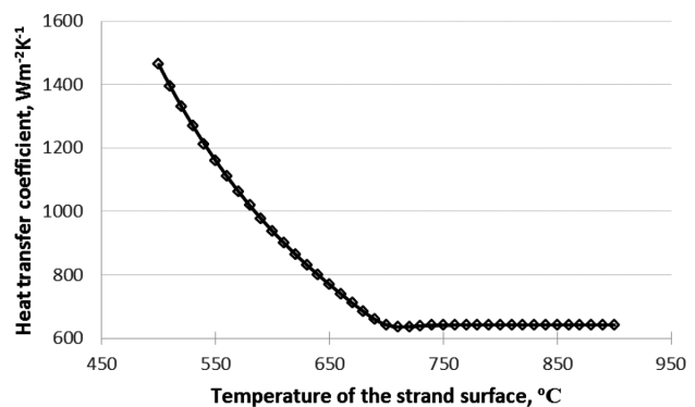
Figure 3: Heat-transfer coefficient during the cooling process with a water spray for \dot{V}_{\text{spray}}^c = 3 \text{ dm}^3 \text{ m}^{-2} \text{ s}^{-1}
