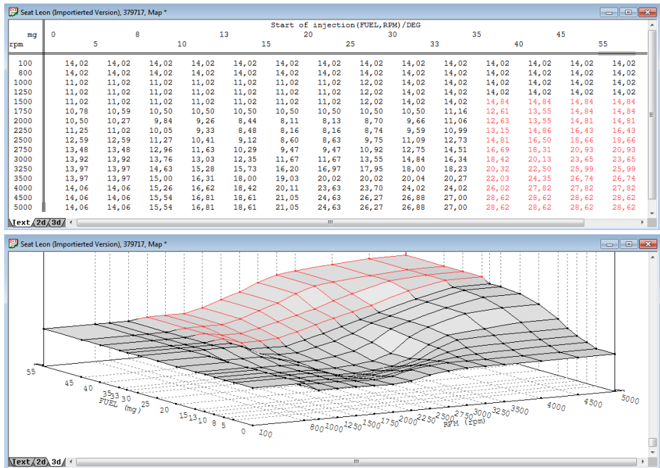
Figure 7: ECONOMY optimization – Start of Injection (Fuel, RPM/DEG)
