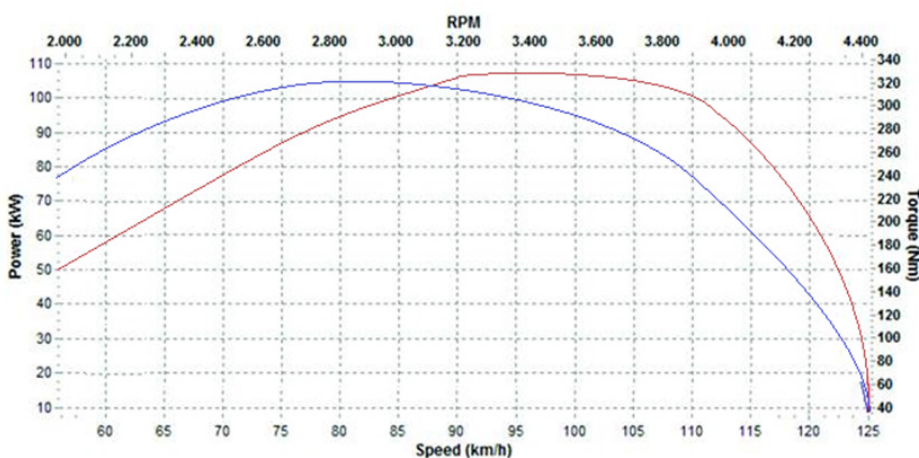
Figure 10: Power output following the POWER optimization
