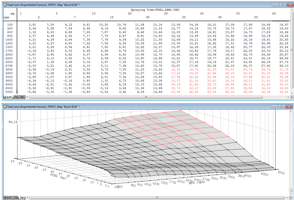
Figure 6: ECONOMY optimization – Injection duration (Fuel, RPM/DEG)
