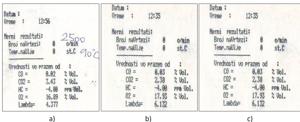
Figure 13: Exhaust emissions: a) Unoptimized; b) Economy; c) Power
