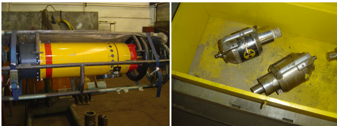
Figure 18: An X-ray machine and defectoscopes used in industrial radiography. (Photo: SNSA inspectorate)
