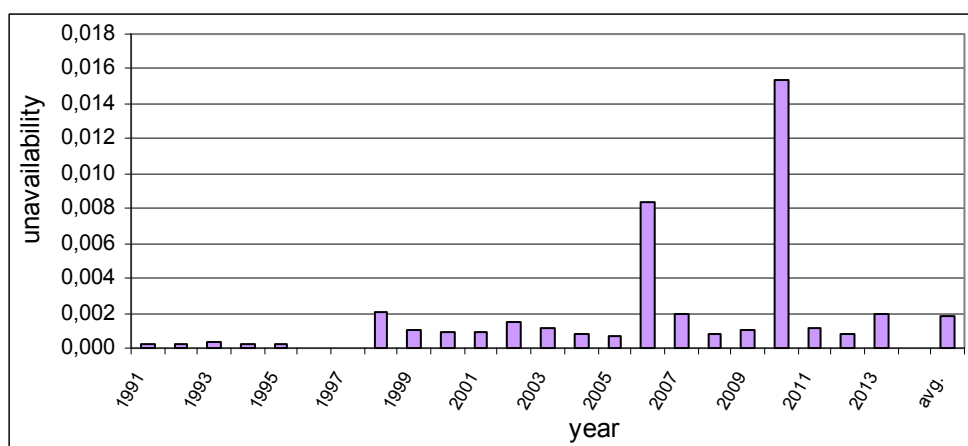
Figure 11: The inoperability of the auxiliary feedwater system
