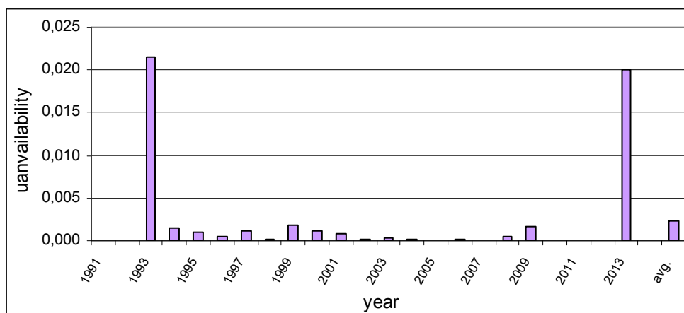
Figure 10: The inoperability of the emergency power supply
