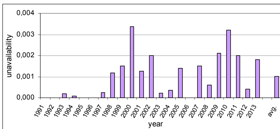
Figure 9: Inoperability of the safety injection system
