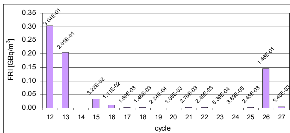
Figure 14: Fuel Reliability Indicator (FRI) for the last 16 fuel cycles
