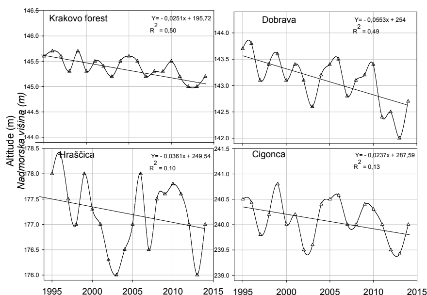
Fig. 4: Dynamics of groundwater table for the observed forest complex - the mean annual value for the closest measuring station is provided.
