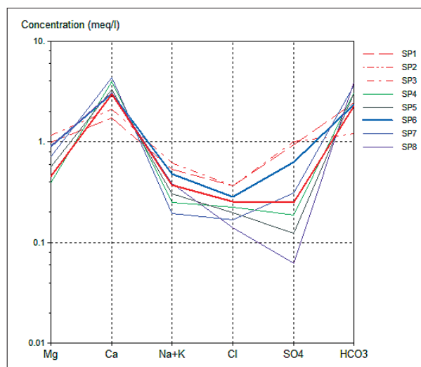
Fig. 6: Semi-logarithmic schoeller diagram of the waters.
