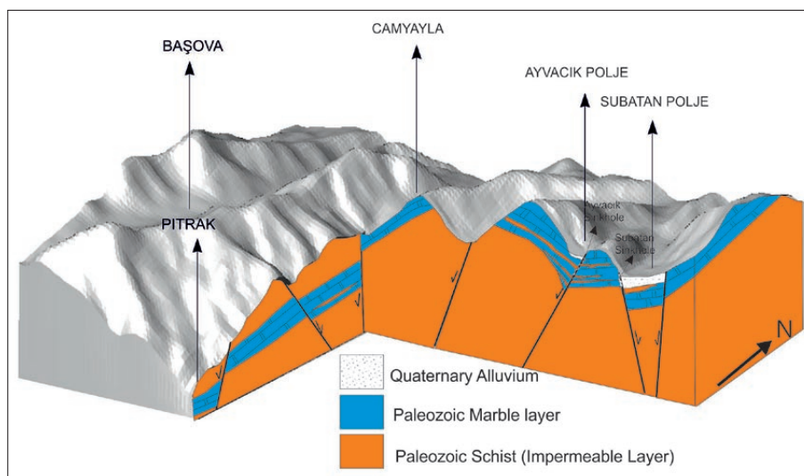
Fig. 3: Geological block diagram of the study area (Simsek et al. 2010).
