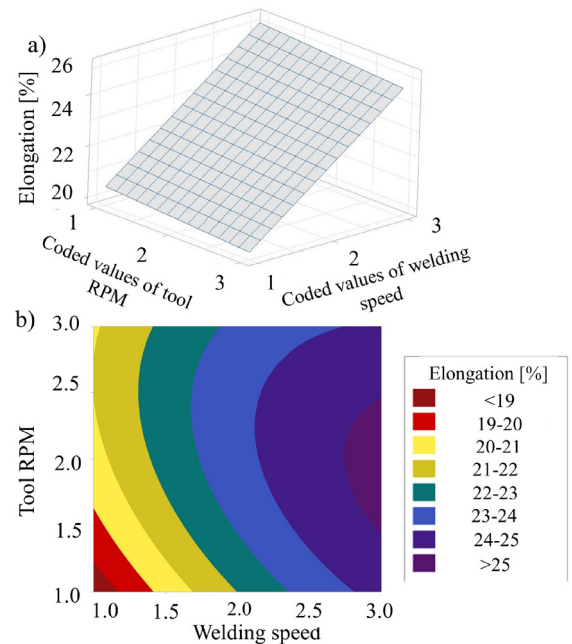
Fig. 5. a) Surface plot showing variation of percentage elongation with the process parameters, and b) contour plot of percentage elongation showing variations with process parameters
