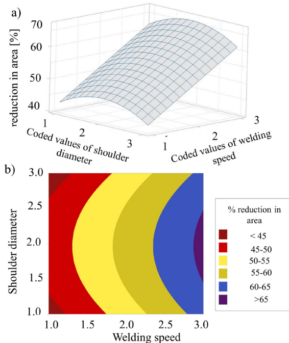
Fig. 6. a) Surface plot showing variation of percentage reduction in area with the process parameters, and b) contour plot of percentage reduction in area showing variations with process parameters
