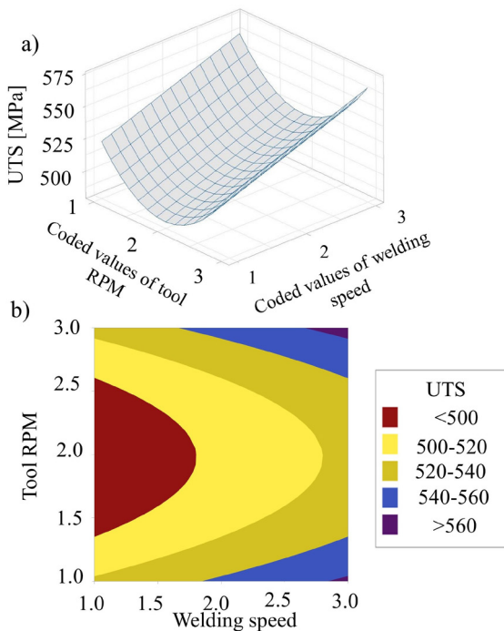
Fig. 4. a) Surface plot showing variation of UTS with the process parameters, and b) contour plot of UTS showing variations with process parameters
