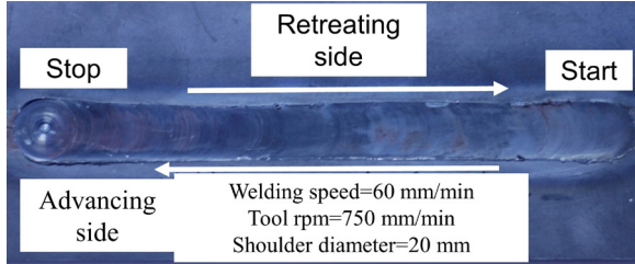
Fig. 1. Photograph of friction stir-welded joint
