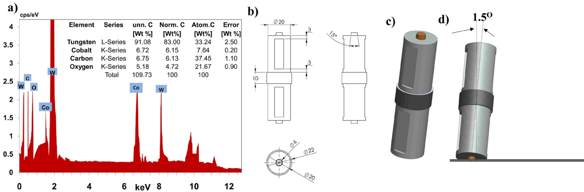
Fig. 2. a) Results obtained from EDAX analysis of tool, b) dimensions of the tool, c) tool profile, and d) 1.5-degree tool tilt angle used in generating the weld samples
