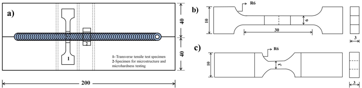
Fig. 3. a) Test coupon for taking out samples for mechanical and metallurgical testing, b) dimensions of transverse tensile test specimen, and c) dimensions of reduced section tensile test specimen
