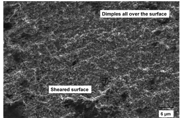
Fig. 10. SEM image of fractured joint region
