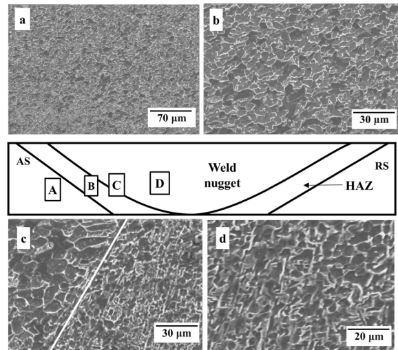
Fig. 7. Optical micrograph of various regions of the friction stir welded steel; a) base metal (region A), b) heat affected zone (region B), c) interface between the heat affected zone and stir zone (region C), and d) stir zone (region D)
