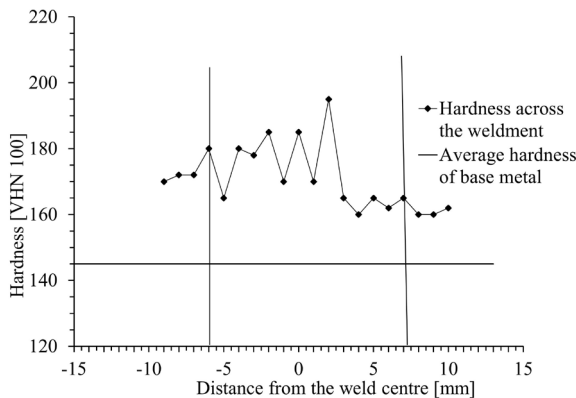
Fig. 9. Microhardness profile (transverse section) of the specimen welded under optimized conditions
