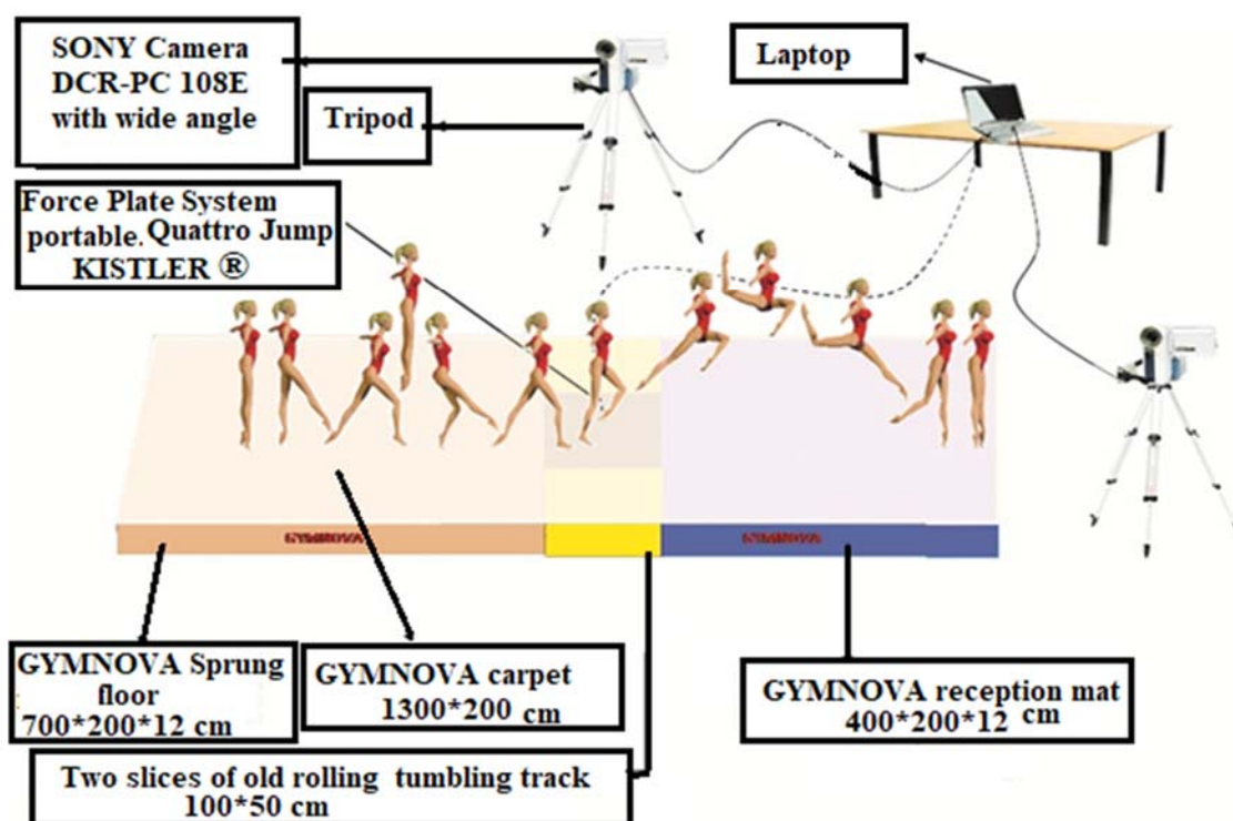
Figure 1. Experimental device.
