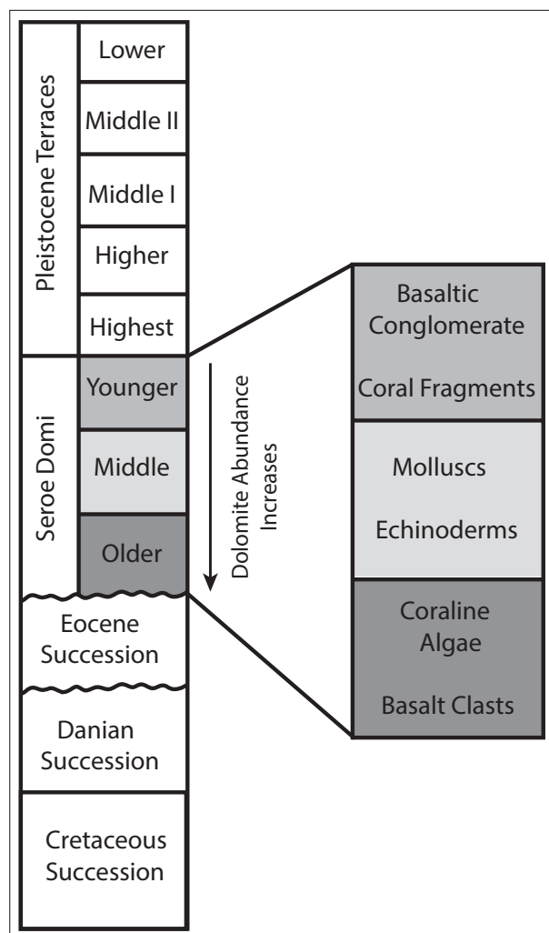
Fig. 2: Generalized stratigraphic column of Curaçao.
