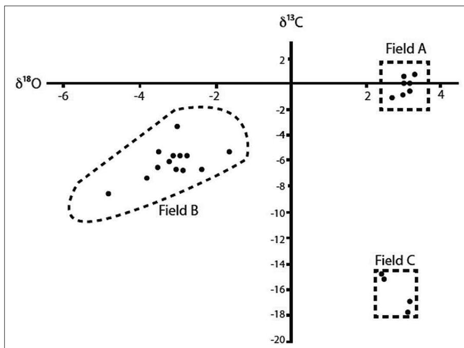
Fig. 9: Plot of \delta^{13}\text{C} (VPDB) vs. \delta^{18}\text{O} (VPDB) of dolomite from the Seroe Domi Formation on Curaçao. Fields A, B and C described in the text.
