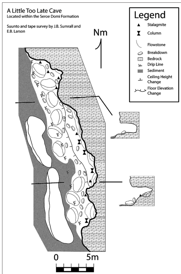
Fig. 11: Map of A Little Too Late Cave (Type 2) located within the Seroe Domi Formation on Curaçao. This cave is interpreted as flank margin in origin based on the morphology and abundance of speleothems. Since the maximum width is the entrance, a majority of the cave has been lost to cliff retreat. This map corresponds to the photograph in Fig. 3B.
