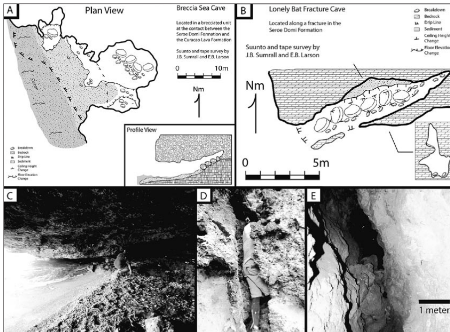
Fig. 13: A) Map of Breccia Sea Cave (Type 5) located at sea level along the contact between the Curaçao Lava Formation and the Seroe Domi Formation on Curaçao. B) Map of Lonely Bat Fracture Cave (Type 4) located along a fracture within the Seroe Domi Formation on Curaçao. C) Photograph within Breccia Sea Cave. D) Entrance to Lonely Bat Fracture Cave. E) Photograph from within Lonely Bat Fracture Cave showing the vertical development and breakdown.
