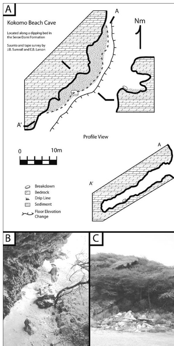
Fig. 12: A) Map of Kokomo Beach Cave (Type 3 cave) located along a dipping bed within the Seroe Domi Formation on Curaçao. B) Photograph along profile of A' to A from the cave map showing a general lack of dissolution morphologies. C) Outcrop view showing that cave formation occurred along the dipping beds of the Seroe Domi Formation.
