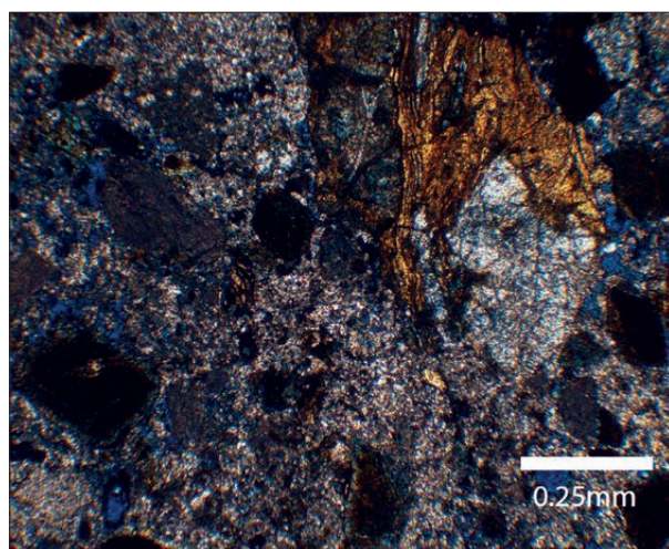
Fig. 7: Thin section micrograph showing dolomitized allochems (dark gray), dolomite cement (clear to white), and clay clasts (light brown). Blue represents porosity filled with blue-dyed epoxy.
