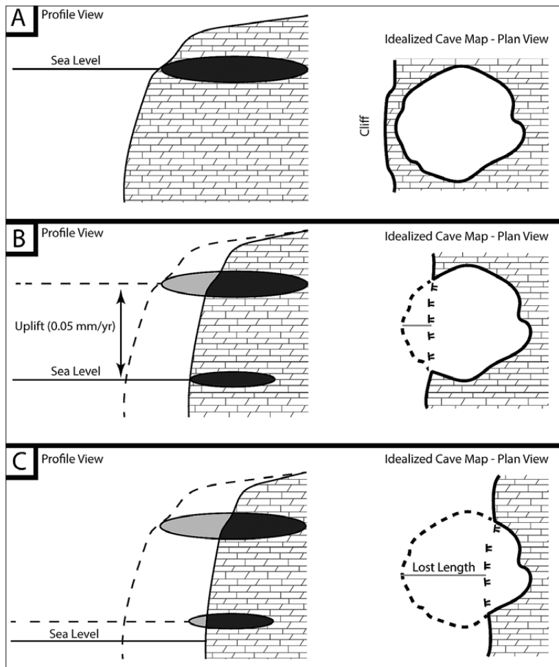
Fig. 14: Idealized cave showing cliff retreat. Uplift from a sea level position of +6m asl is calculated using the rate 0.05mm/yr. The idealized cave map in plain view of the upper cave is shown on the right of each panel. Originally flank margin caves form as entrance-less caves. Cave entrances are the result of breaching by cliff retreat and denudation. When the entrance width is the maximum width, the cave is considered to be at least half lost to cliff retreat. By first establishing cliff retreat rates, lost length can be estimated and original void area can be calculated.
