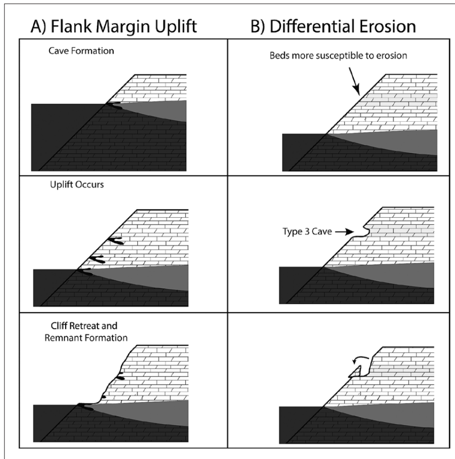
Fig. 15: A) Genetic model for the formation of remnant flank margin caves (Type 2). Other cave types that form at sea level (such as sea caves) would follow a similar process; however, only flank margin caves appear to survive the duration of cliff retreat experienced by higher elevation caves. B) Differential erosion model showing the development of Type 3 caves and how these caves are “lost” due to erosion undercutting the resistant overlying beds.
