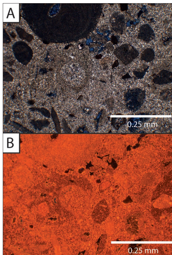
Fig. 8: A) Thin section micrograph showing a dolomitized grainstone. Blue represents porosity filled by blue-dyed epoxy. B) Cathodoluminescence micrograph of the same field as (A) showing two types of luminescence. Dolomite pore-filling cements appear zoned. The red algae allochem in the top left corner of micrograph (A) cannot be distinguished from the matrix by cathodoluminescence in (B).
