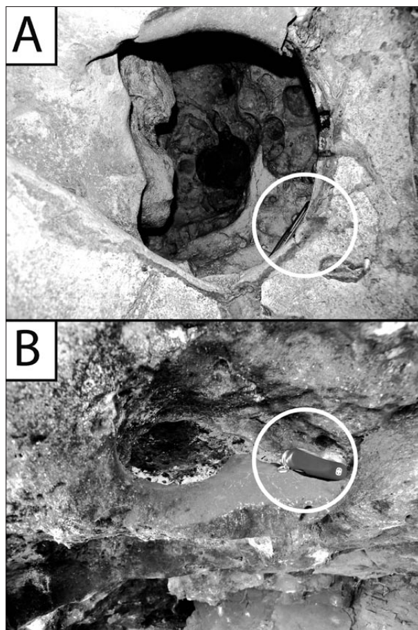
Fig. 6: Dissolution pockets that penetrate into the ceiling (A) and wall (B) of the carbonate unit at the basalt-carbonate contact. Circles are around a pocketknife approximately 6 centimeters in length.
