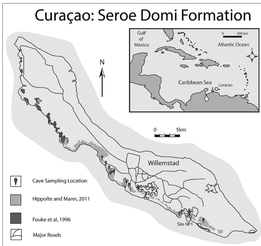
Fig. 1: Location map showing sampling sites from outcrop and caves located within the Seroe Domi Formation. The shaded regions on the southern coast correspond to dolomitized outcrops of the Seroe Domi Formation, as mapped by Hippolyte & Mann (2011) and Fouke et al. (1996).
