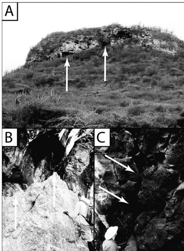
Fig. 5: An outcrop showing caves (Type 1) that formed near and slightly above the basaltic diabase and carbonate contact on Curaçao. A) Remnant caves had undulating ceilings, and caves do not follow lithologic contacts. Vertical extent of photograph is 35 meters. Arrows point to typical caves. B) The basaltic diabase contact has an irregular weathering surfaces indicated by the arrow. This contact is the unconformity between the Cretaceous succession and the Seroe Domi Formation. C) Extensive fracture networks penetrating into the overlying carbonate unit were associated with caves (arrows).
