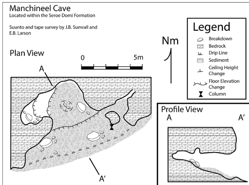
Fig. 10: Map of Manchineel Cave (Type 2) located within the Seroe Domi Formation on Curaçao. This cave is interpreted as flank margin in origin based on morphology. This map corresponds to the photograph in Fig. 3A.
