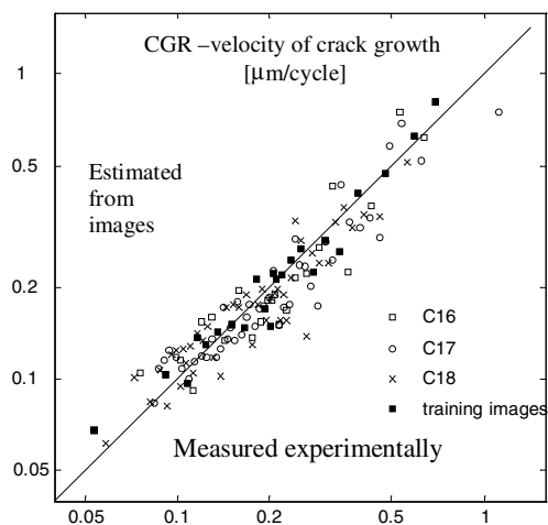
Fig. 6. Comparison of crack growth rates measured experimentally and estimated on the basis of training images. One point represents one image. The line y = x represents the ideal agreement.
