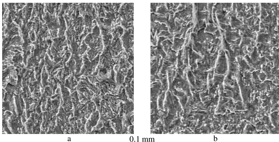
Fig. 1. Examples of typical textures in images of fatigue crack surface. Low (a) and high (b) crack growth rate. Stainless steel AISI 304L.
