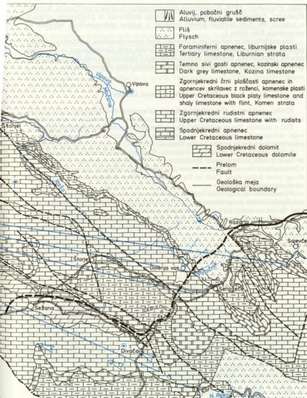
Fig. 1. Hydrogeological map of Kras (after geological map 1:100 000, sheet Postojna, 1967; sheet Gorica, 1968)
