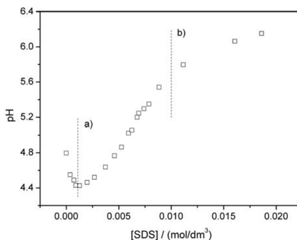
Figure 5. pH of 1.0 \times 10^{-3} \text{ mol/dm}^3 \text{ Al(NO}_3)_3/\text{SDS} mixed aqueous solutions at 298.15 \text{ K} . a) [\text{SDS}] = 1.1 \times 10^{-3} \text{ mol/dm}^3 , and b) [\text{SDS}] = 10 \times 10^{-3} \text{ mol/dm}^3 .
