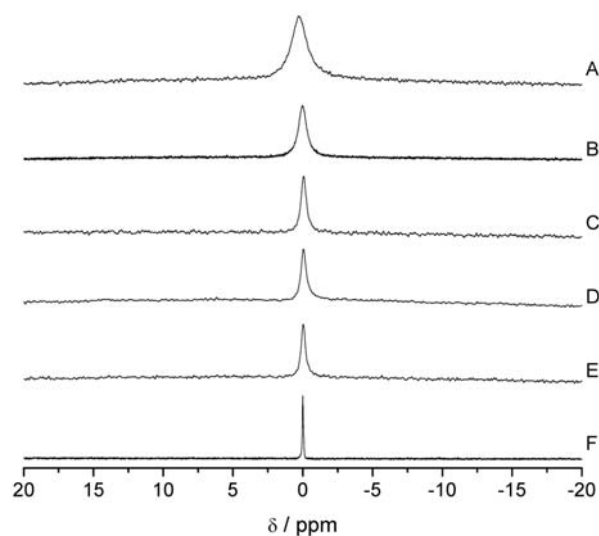
Figure 2. ^{27}\text{Al} NMR spectra of different mixed Al(III) 1.079 mmol/kg:SDS \text{D}_2\text{O} solutions: A) [SDS] = 0 mol/dm 3 ; B) [SDS] = 0.41 \times 10^{-3} mol/dm 3 ; C) [SDS] = 2.80 \times 10^{-3} mol/dm 3 ; D) [SDS] = 4.87 \times 10^{-3} mol/dm 3 ; E) [SDS] = 5.91 \times 10^{-3} mol/dm 3 ; and F) [SDS] = 0 and pH = 2.
