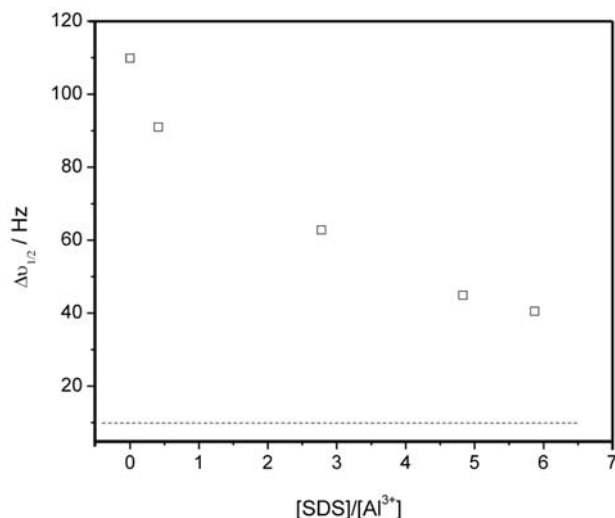
Figure 3. Dependence of the half-height linewidth ( \Delta v_{1/2} ) on the SDS concentration in the ^{27}\text{Al} NMR spectra of 1.01 \times 10^{-3} \text{ mol/dm}^3 \text{Al(III)/SDS} solutions. Dashed line shows the \Delta v_{1/2} of \text{Al(III)} at pH 2.
