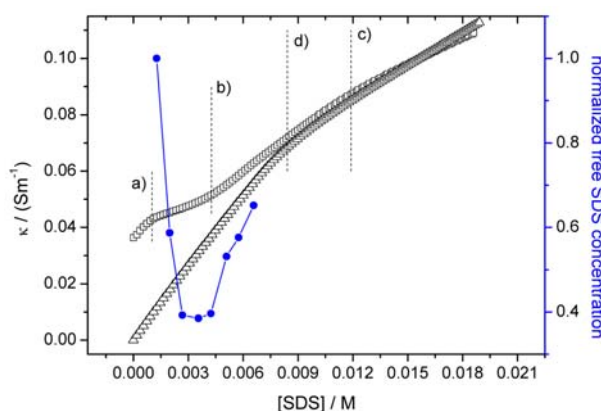
Figure 4. Specific electrical conductance, \kappa , (open symbols) and normalised free concentration (full symbols) as measured by selective electrode potentiometry (o) of SDS in water ( \Delta ) and in aqueous solution of 1 \text{ mM Al(NO}_3)_3 at 298.15 \text{ K} . Vertical dashed lines show inflexion points as seen by electrical conductivity: a) [\text{SDS}] = 1.01 \times 10^{-3} \text{ mol/dm}^3 ; b) [\text{SDS}] = \text{mic} = 4.27 \times 10^{-3} \text{ mol/dm}^3 ; c) [\text{SDS}] = \text{cmc}^{\text{ap}} = 11.9 \times 10^{-3} \text{ mol/dm}^3 ; d) [\text{SDS}] = \text{cmc} = 8.42 \times 10^{-3} \text{ mol/dm}^3 .
