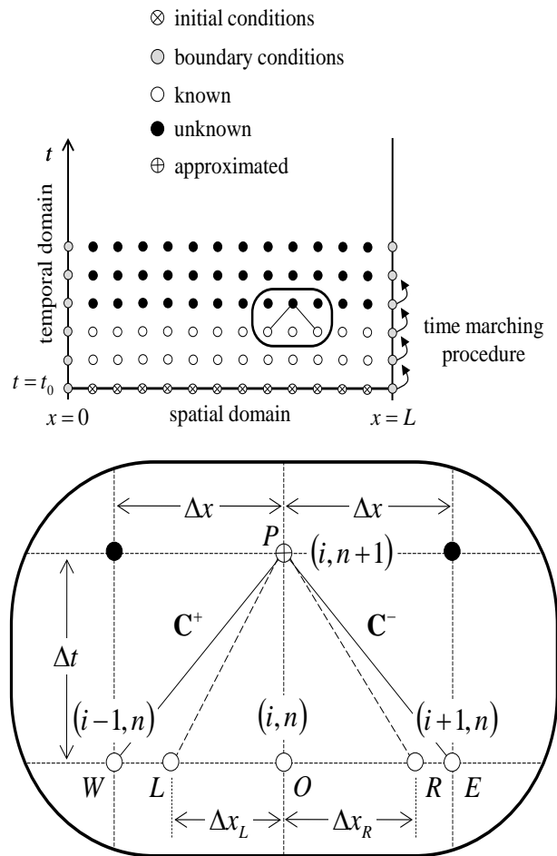
Figure 1: Staggered space-time grid used in MOC.
