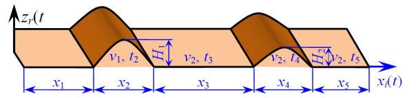
Fig. 5. Ground excitation represented by double cosine road bumps
