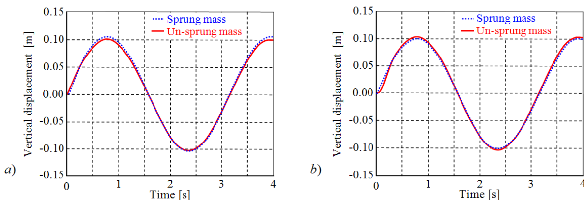
Fig. 7. Simulation of the displacements of the sprung and un-sprung masses, performed by a) WM and b) MATLAB platforms
