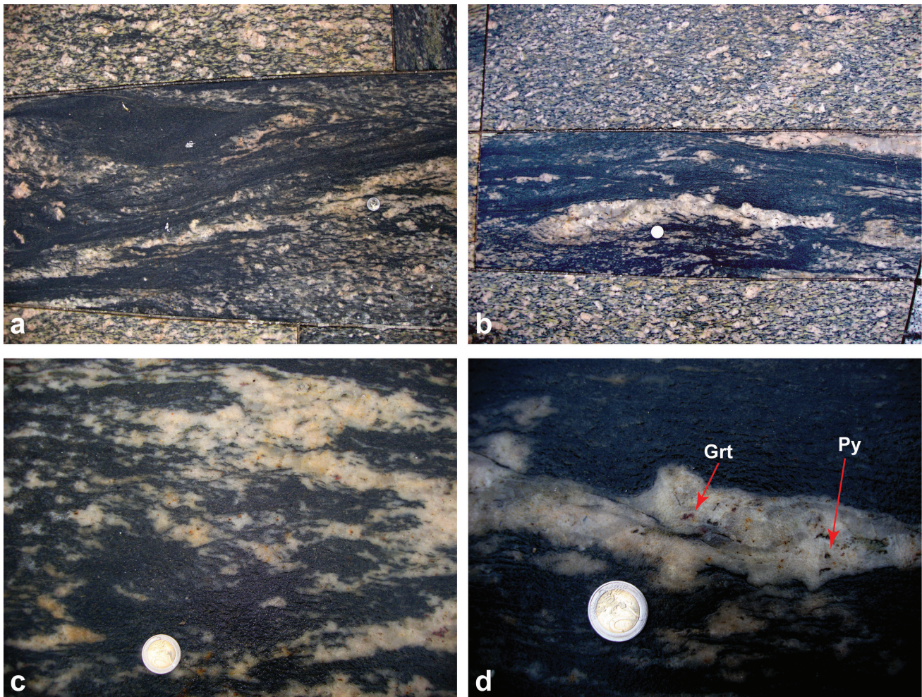
Fig. 5. Dark coloured pavers used in central courtyard of Ljubljana Castle. (a–b) Typical gneissic structure and contrast of dark pavers in contact with light coloured varieties (top and bottom border). (c) Most minerals in dark coloured pavers are macroscopically indistinguishable. (d) Reddish minerals in the felsic lens composed of white feldspars and quartz correspond to garnets (Grt), dark spots are pyrite (Py).
