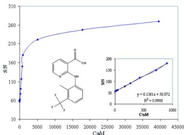
Figure 6. Calibration curves obtained for flunixin on the Au microelectrode in 0.05 M \text{H}_3\text{PO}_4 .
