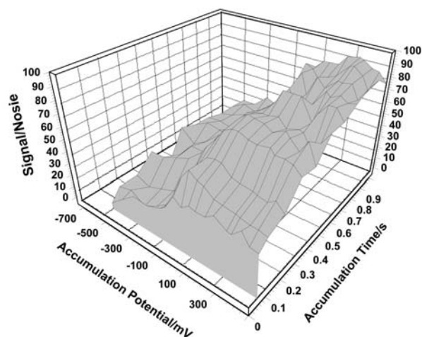
Figure 5. The effect of accumulation potential and the effect of accumulation time on the electrode response to injections of 5.0 \times 10^{-7} M flunixin in 0.05 M \text{H}_3\text{PO}_4 .
