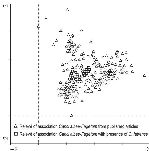
Figure 2: Association Carici albae-Fagetum , 185 selected relevés from already published articles, 26 relevés with presence of the Cyclamen fatrense . Detrended correspondence analysis, each point represents one relevé.
