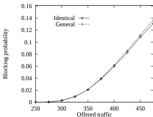
Figure 16: Blocking probabilities for the NSFNET topology of Fig. 2 with link parameters of Table 3; nonuniform load, 2 & 3 hops away SD pairs.
