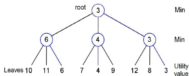
Figure 1: Minimin search.
