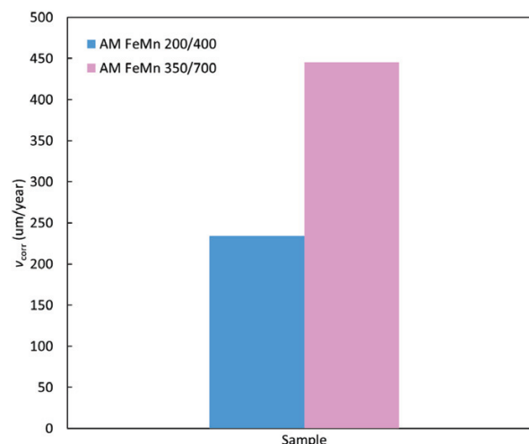
Figure 5: Corrosion rates calculated from potentiodynamic measurements for AM FeMn 200/400 sample (laser power 200 W, scanning speed 400 mm/s) and AM FeMn 350/700 sample (laser power 350 W, scanning speed 700 mm/s) measured in Hank's solution
