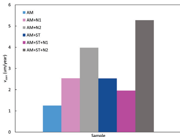
Figure 4: Corrosion rates calculated from potentiodynamic measurements for AM as-built (AM), as-built + nitrided at 430 °C/15 h (AM + N1), as-built + nitrided at 500 °C/15 h (AM + N2), as-built + solution treated 1050 °C/1 h (AM + ST), as-built + solution treated 1050 °C/1 h + nitrided at 430 °C/15 h (AM + ST + N1) and as-built + solution treated 1050 °C/1 h + nitrided at 500 °C/15 h (AM + ST + N2)
