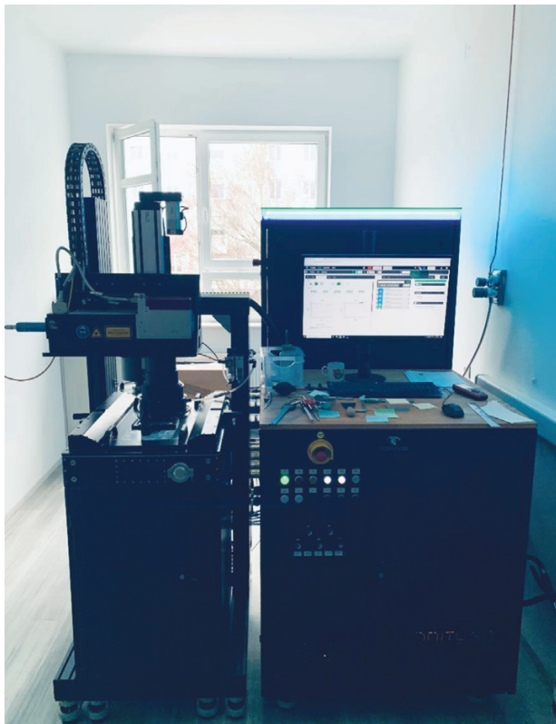
Figure 1: SLM Aconity3D MINI instrument equipped with 800 °C preheating option, installed at the Institute of Metals and Technology
