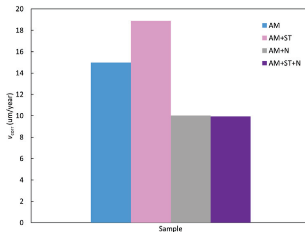
Figure 3: Corrosion rates calculated from potentiodynamic measurements for AM as-built 18Ni-300 maraging steel (AM), after aging treatment at 520 °C for 6 h (AM + ST), after nitriding at 520 °C for 6 h (AM + N) and after aging treatment at 520 °C for 6 h and nitriding (AM + ST + N)
