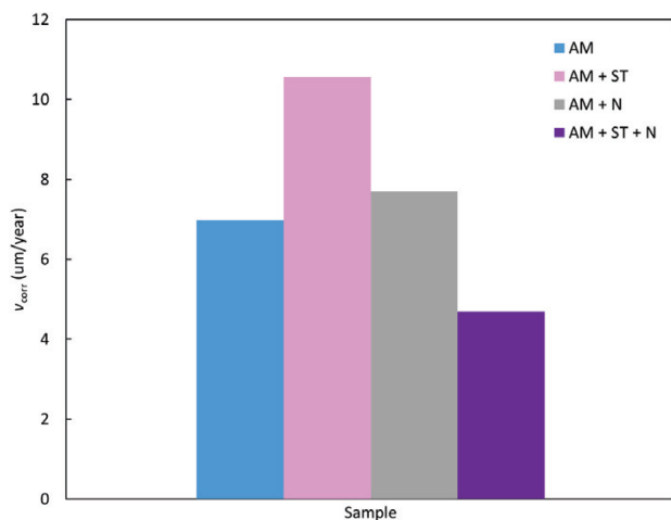
Figure 2: Corrosion rates calculated from potentiodynamic measurements for AM 316 L as-built (AM), nitrided at 430 °C for 15 h (AM + N), solution treated at 1060 °C for 30 min (AM + ST) and solution treated and nitrided (AM + ST + N) in 3.5 % NaCl
