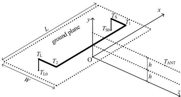
Figure 4: Simplified CISPR25 geometry used for radiated emissions calculations
