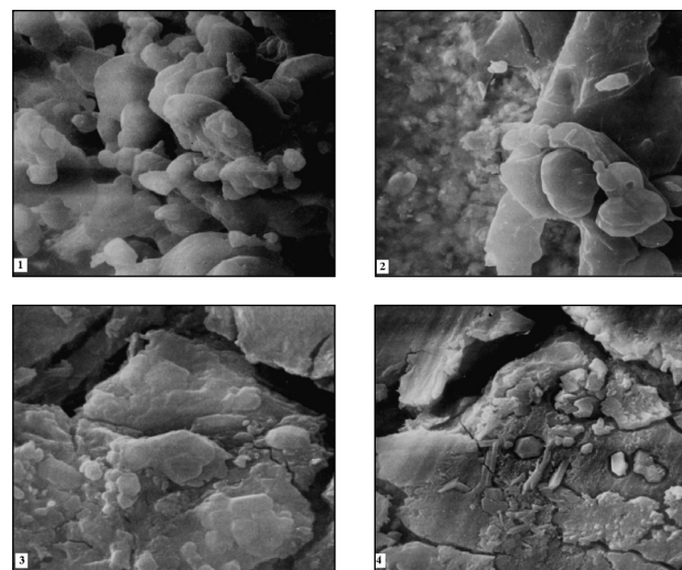
Figure 8. Scanning electron micrographs of \text{Na}_2\text{B}_4\text{O}_7 \cdot 10\text{H}_2\text{O} recorded at 25 °C: before and after irradiation: 1 – 0, 2 – 1, 3 – 4 and 4 – 8 hours. Magnifications 15000 X.
