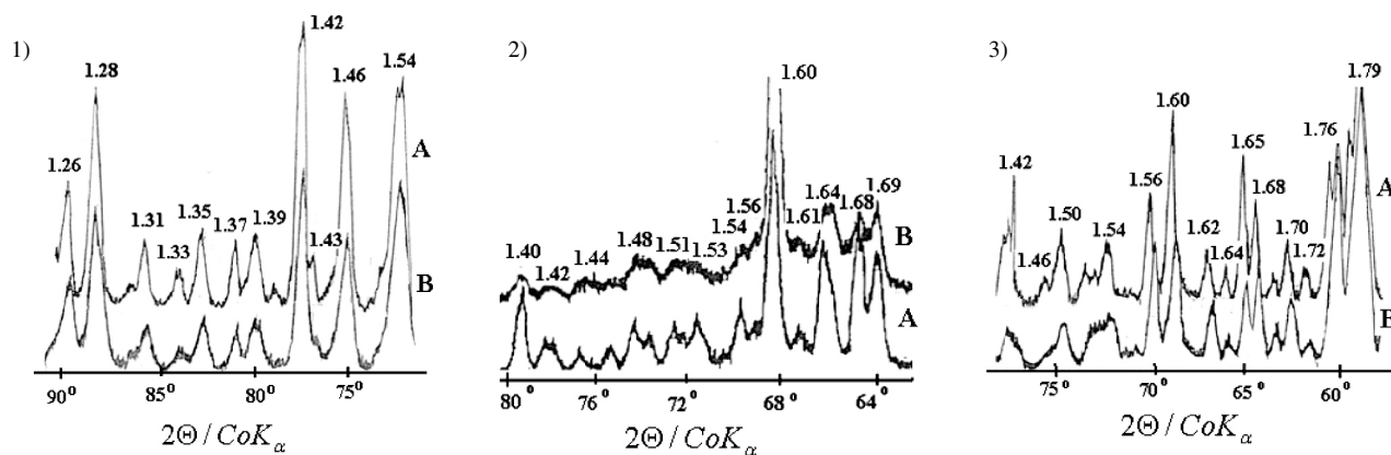
Figure 2. Characteristic part of the X-ray diffraction patterns 1 – \text{Li}_2\text{CO}_3 recorded at 25 ^\circ\text{C} : A – before and B – after irradiation 8 hours, 2 – \text{H}_3\text{BO}_3 recorded at 25 ^\circ\text{C} : A – before and B – after irradiation 2 hours, 3 – \text{Na}_2\text{B}_4\text{O}_7 \cdot 10\text{H}_2\text{O} recorded at 25 ^\circ\text{C} : A – before and B – after irradiation 8 hours.
