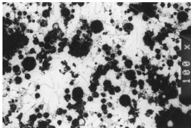
Figure 1: Photomicrograph of A356- 22.8 vol.% dross particles
