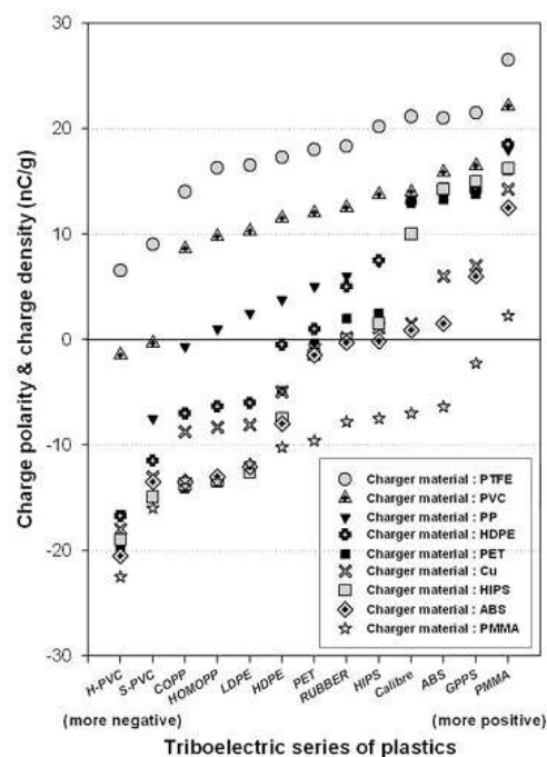
Fig. 3. Triboelectric series of various plastics established by the tribo-charging of different combinations of two plastics.
