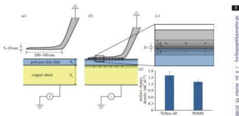
Figure 2. (a) Before contact of a nano-spatula—at the tip of a seta of a gecko toe pad—with the polymer thin film, both the spatula and the thin film were electrically neutral. (b) As the toe pad came into contact with the polymer thin film, electric charges separated between the nano-spatula and the thin film. The EDL, which was formed at the contact interface, induced certain electric charges in the backing copper sheet, which was grounded through an electrometer. (c) Electric charges that separated upon contact penetrated up to a depth of d_f and d_s into the polymer thin film and the contacted nano-spatula, respectively. D is the actual separation distance (approx. 0.3 nm) [7,21] between the nano-spatula and the thin film. (d) Surface charge densities measured right after contact of gecko toe pads with Teflon AF and PDMS. (Online version in colour.)
