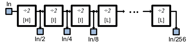
Figure 2: Structure of divide-by-N frequency divider. \div 2 [H]– divideby2 divider working at highest frequency, \div 2 [I]– divideby2 divider working at intermediate frequency, \div 2 [L]– divideby2 divider working at low frequency. In – input signal, In/N– input signal divided by N, where N = 2, 4, 8, 16, 32, 64, 128, 256
