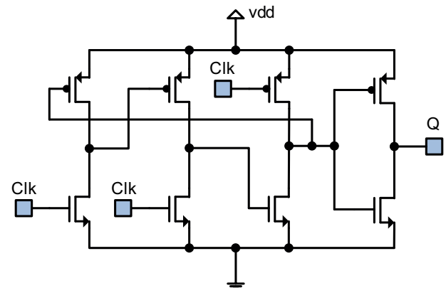
Figure 3: Structure of ETSPC divide-by-2 frequency divider. Clk – input signal. Q – divided by 2 output signal
