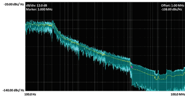
Figure 7: The measured phase noise, when V_{\text{tune}} = 2.5 \text{ V} and the switched capacitor block code = 0
