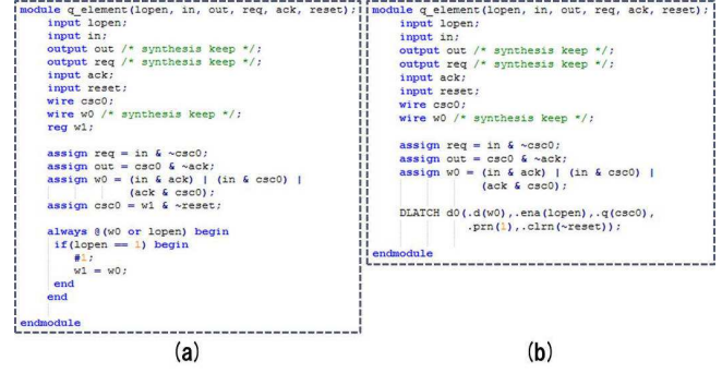
Figure 10: Verilog HDL models of an asynchronous processor: (a) simulation model and (b) synthesis model.
