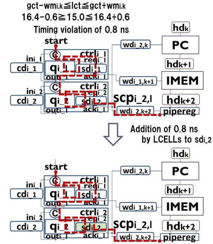
Figure 14: Delay adjustment for simultaneous writing constraints.
