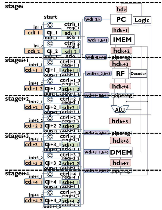
Figure 2: An asynchronous processor model with bundled-data implementation.
