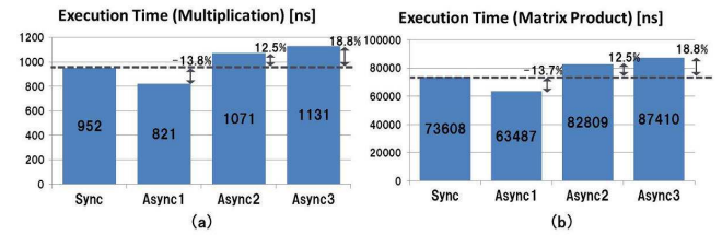
Figure 18: Execution time of MIPS processors: (a) multiplication and (b) matrix multiplication.
