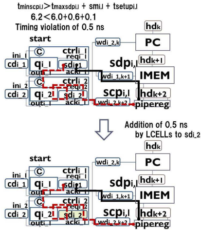
Figure 15: Delay adjustment for a setup constraint.
