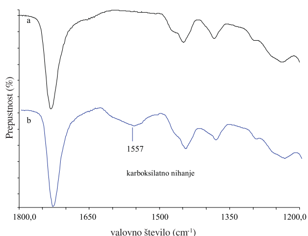
Slika 5: IR-spektra vodne raztopine kopolimera: a) s 6% AK; b) s 6% AK in ZnO Figure 5: IR spectra of water copolymer solution: a) with 6% AA; b) with 6% AA and ZnO
