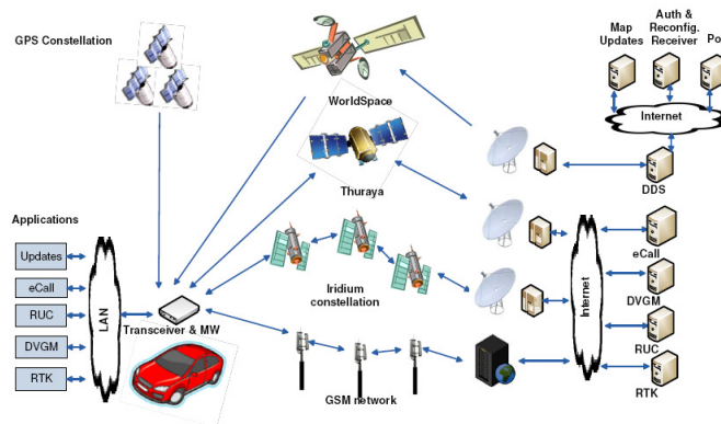
Figure 2 SISTER architecture
