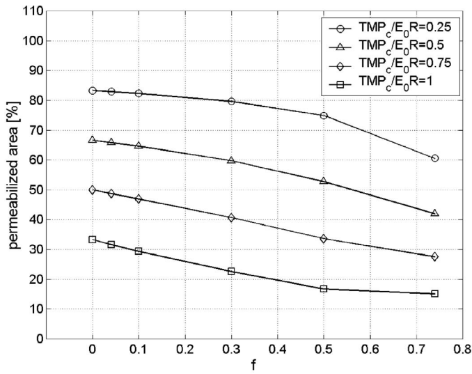
Fig. 5. Percentage of permeabilized area for fcc lattice for different normalized critical TMPs. For \text{TMP}_c/E_0R given in range reported in literature (0.25–1 V) and for a typical cell size ( R \sim 10 \mu\text{m} ) is E_0 \sim 100 \text{ kV/m} . For f = 0 , we have the case of an isolated cell.
