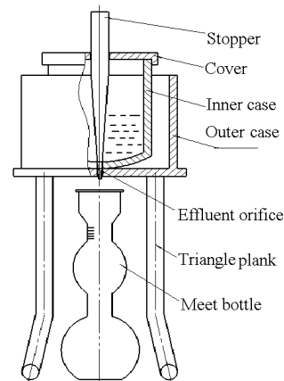
Fig. 4. Experimental set-up for (CH_3)_3SiO[Si (CH_3)_2O]_n Si (CH_3)_3 viscosity
