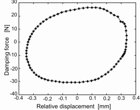
Fig. 5. Damping force variations sine excitation, frequency of 10Hz
