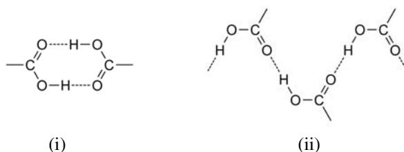
Scheme 1. Hydrogen bond synthons of carboxylic acids: a dimer (i) and a catemer (ii).
