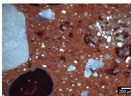
4. A thin section of Sample 2. XPL with Zeiss Axio-cam 305 color.
