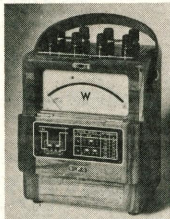
Nekoč in danes, staro in novo; prenosni wattmeter EL 3 (levo) in iskrascope LCD (desno).
