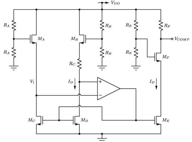
Figure 2: Compensation circuit
