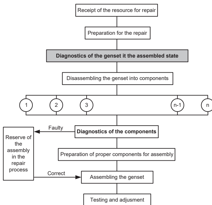
Figure 1: Schematic of the technological process on the principle of repairing a set
